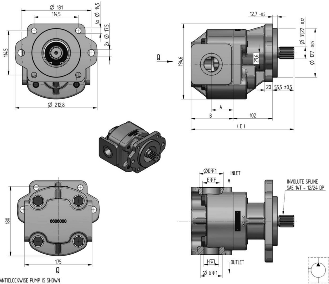
ANTICLOCKWISE PUMP IS SHOWN
