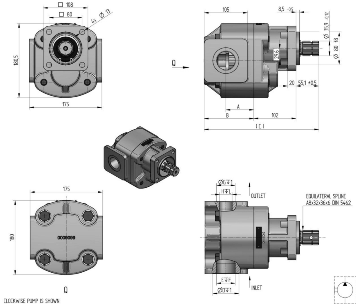
CLOCKWISE PUMP IS SHOWN
